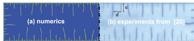
Numerical simulation of a ceramic slab submitted to a thermal shock by a gradient damage model (a) Computed damage field d (blue, d=0 ; red, d=1 ). (b) Experimental results from [20]: Y. Shao, Y. Zhang, X. Xu, Z. Zhou, W. Li, and B. Liu, J. Am. Ceram. Soc. , 94: 2804, 2011.
